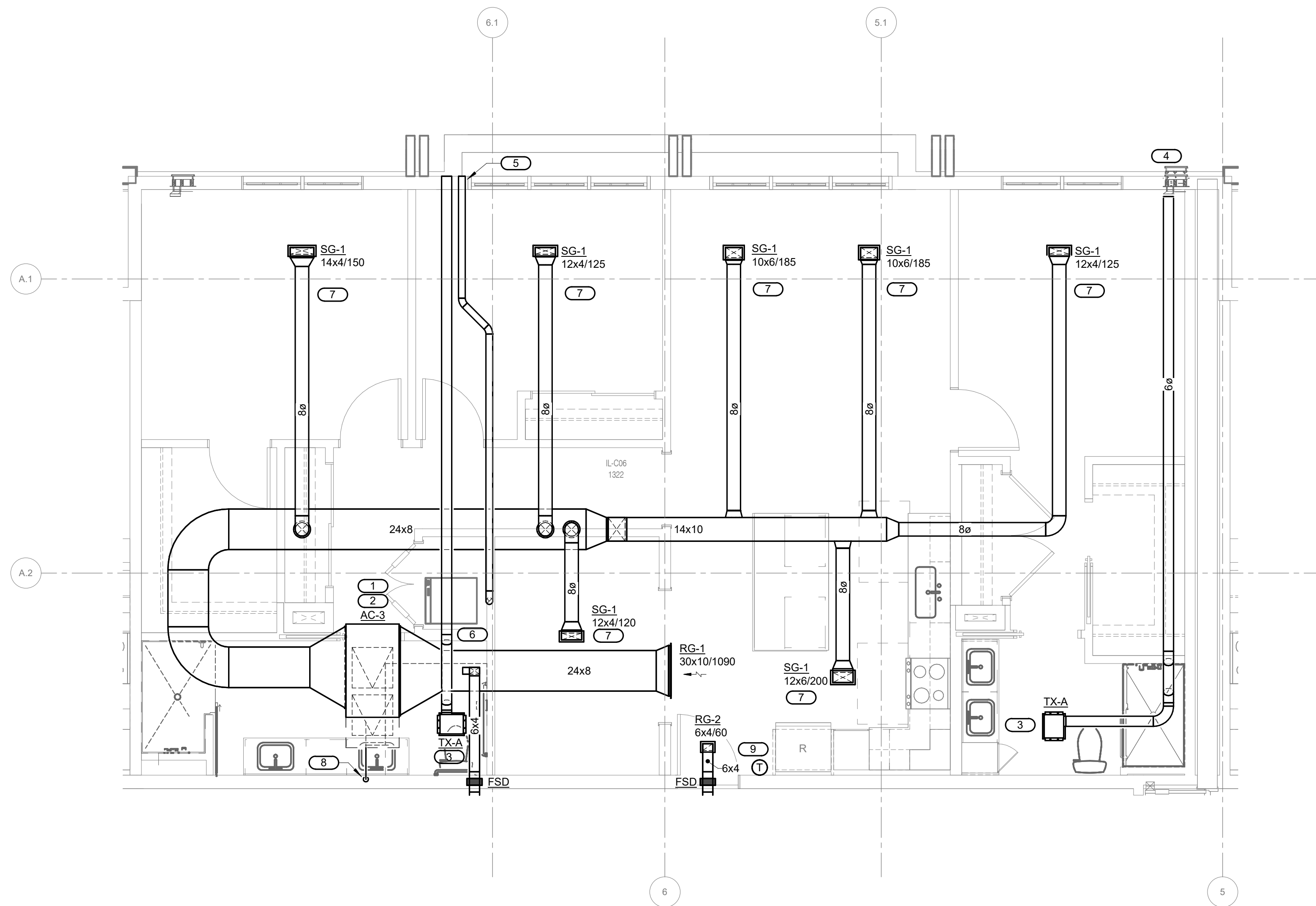
3 MECH. UNIT C06 - 3 BED 2 BATH + DEN - PLAN 1/4" = 1'-0"
