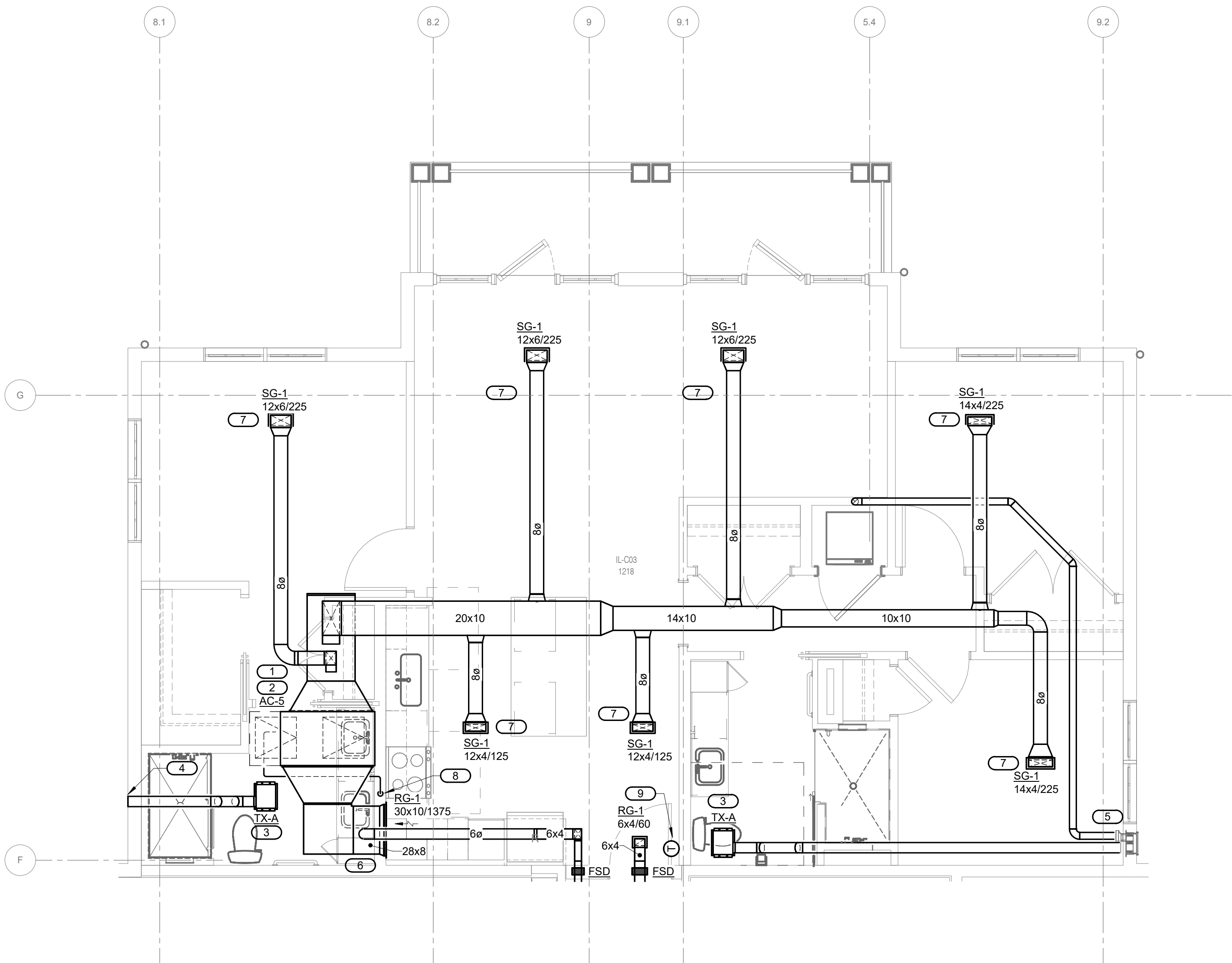
3 MECH. UNIT C03 - 3 BED 2 BATH - PLAN - AC-5 1/4" = 1'-0"
