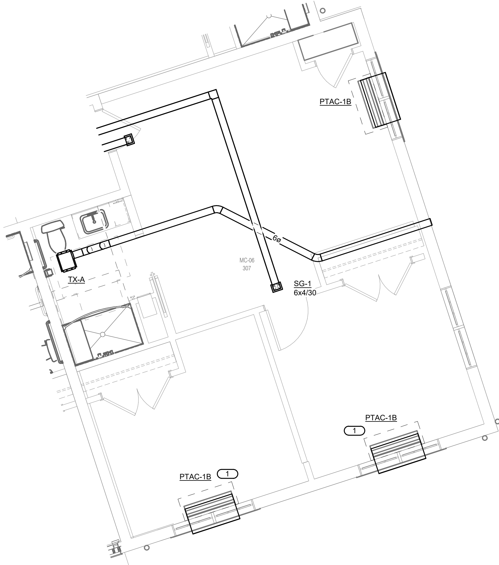
2 MECH. REM SEMI-PRIVATE - (NORTH-EAST) CORNER UNIT - MC-06 1/4" = 1'-0"
