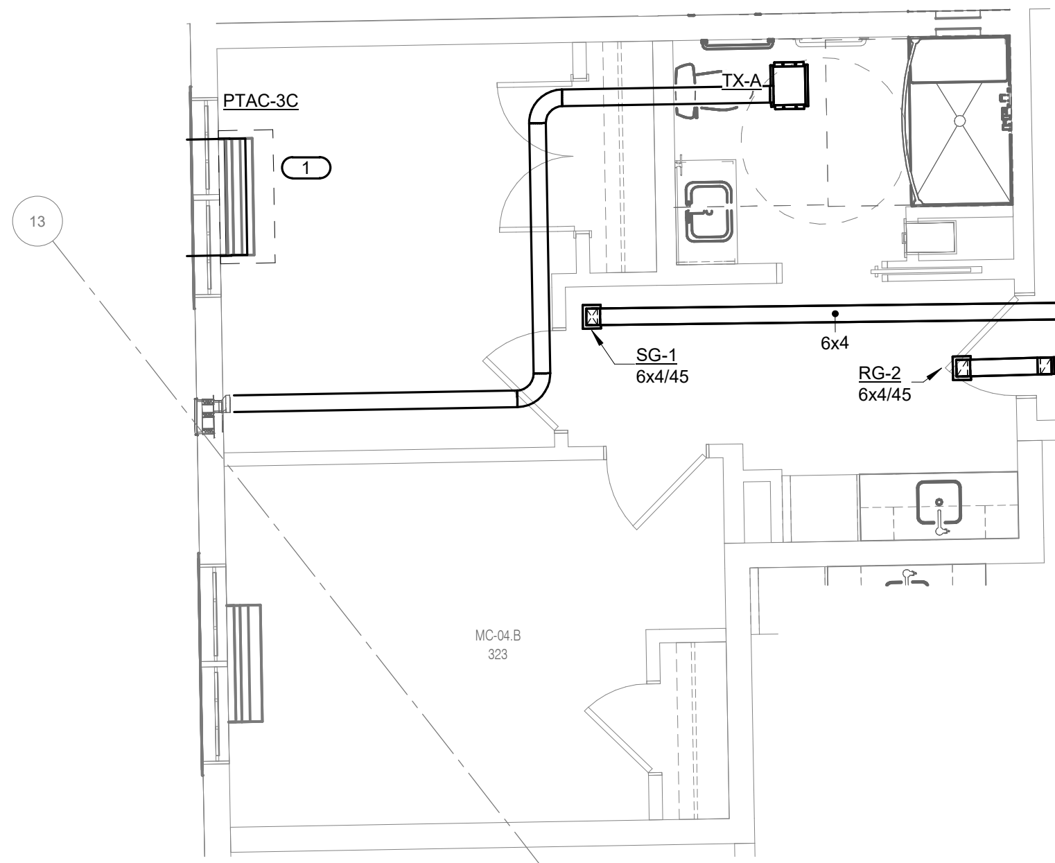
6 MECH. MC-04.B 1/4" = 1'-0"
