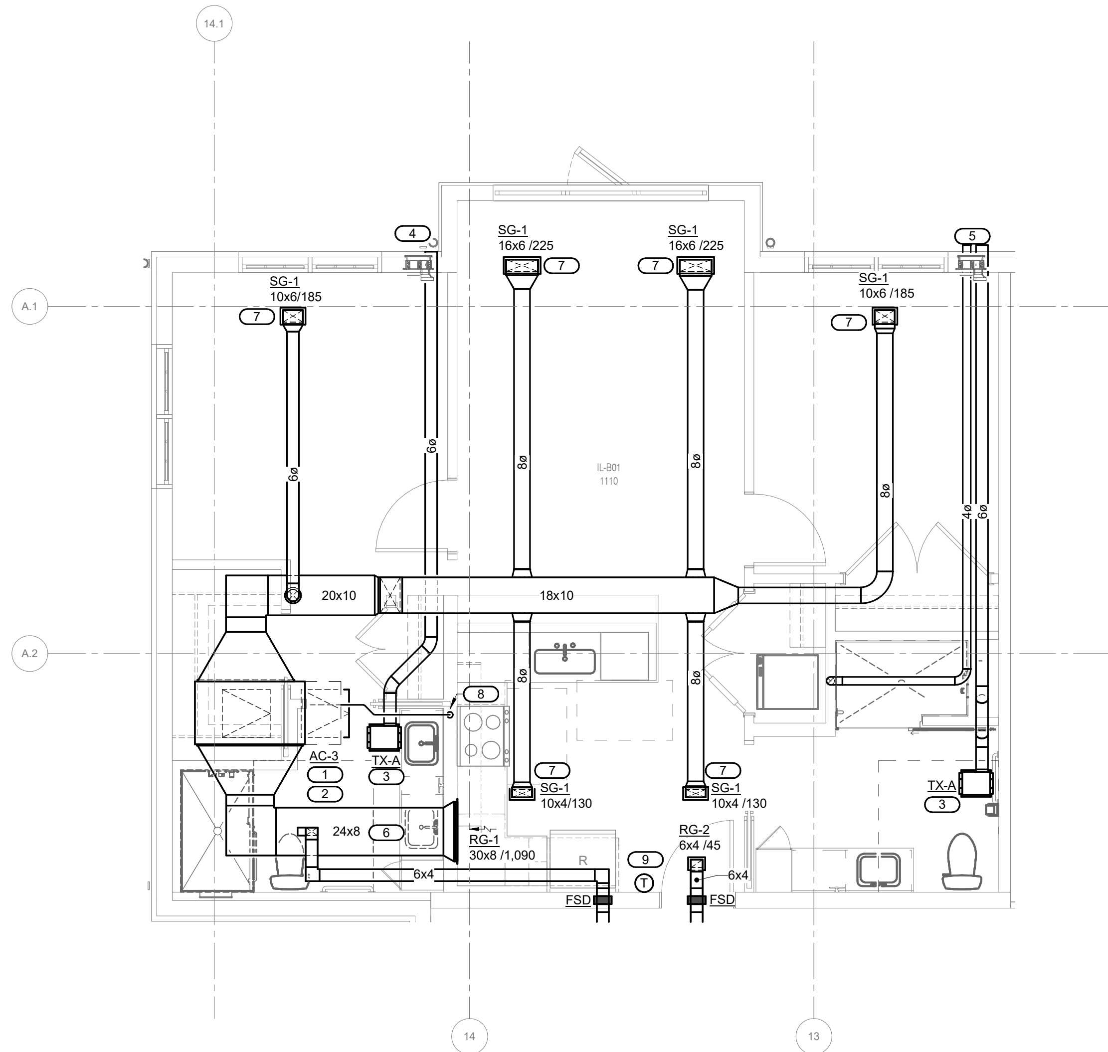
3 MECH. UNIT B01 - 2 BED 2 BATH - PLAN - AC-3 - FIRST FLOOR 1/4" = 1'-0"
