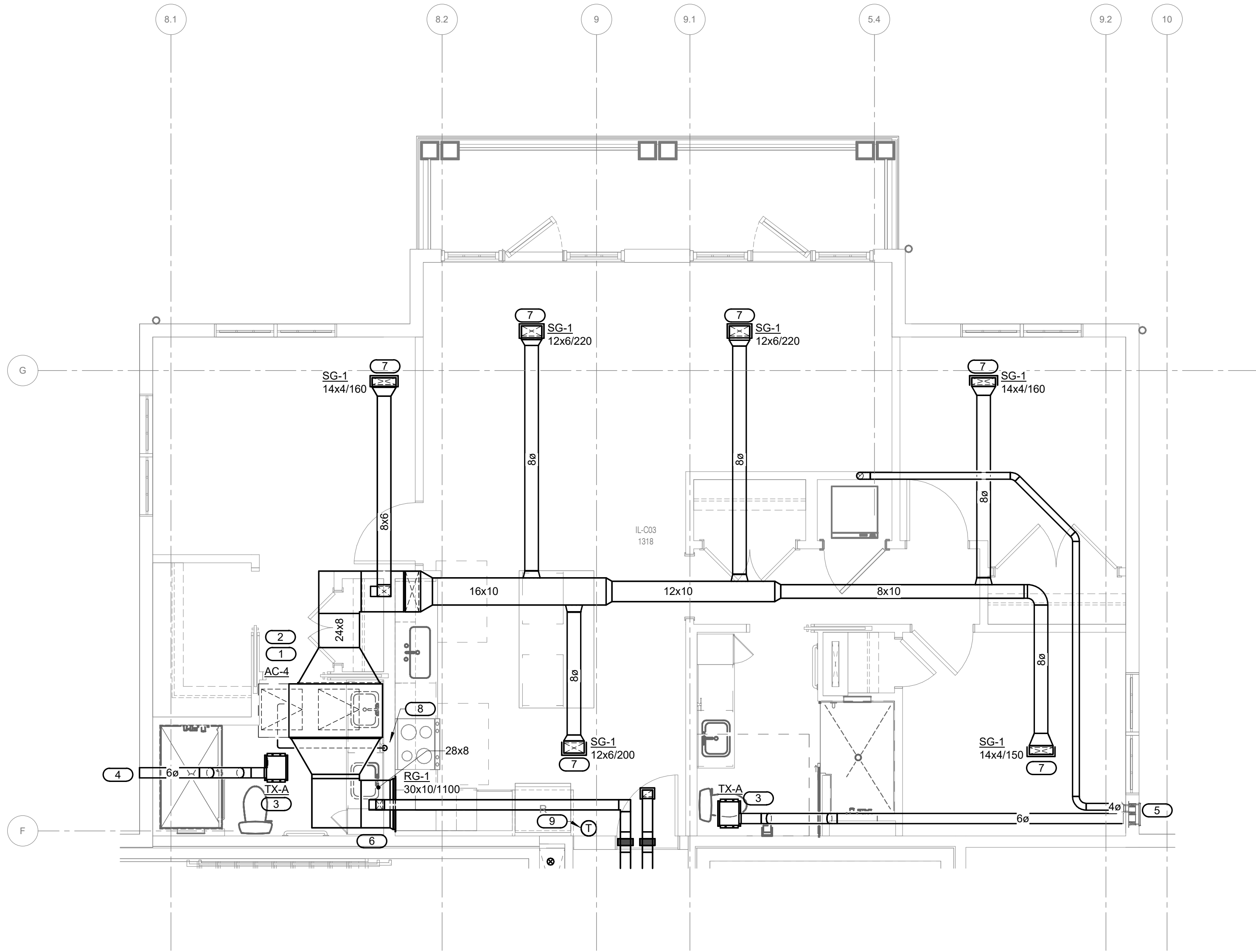
2 MECH. UNIT C03 - 3 BED 2 BATH - PLAN - AC-4 1/4" = 1'-0"
