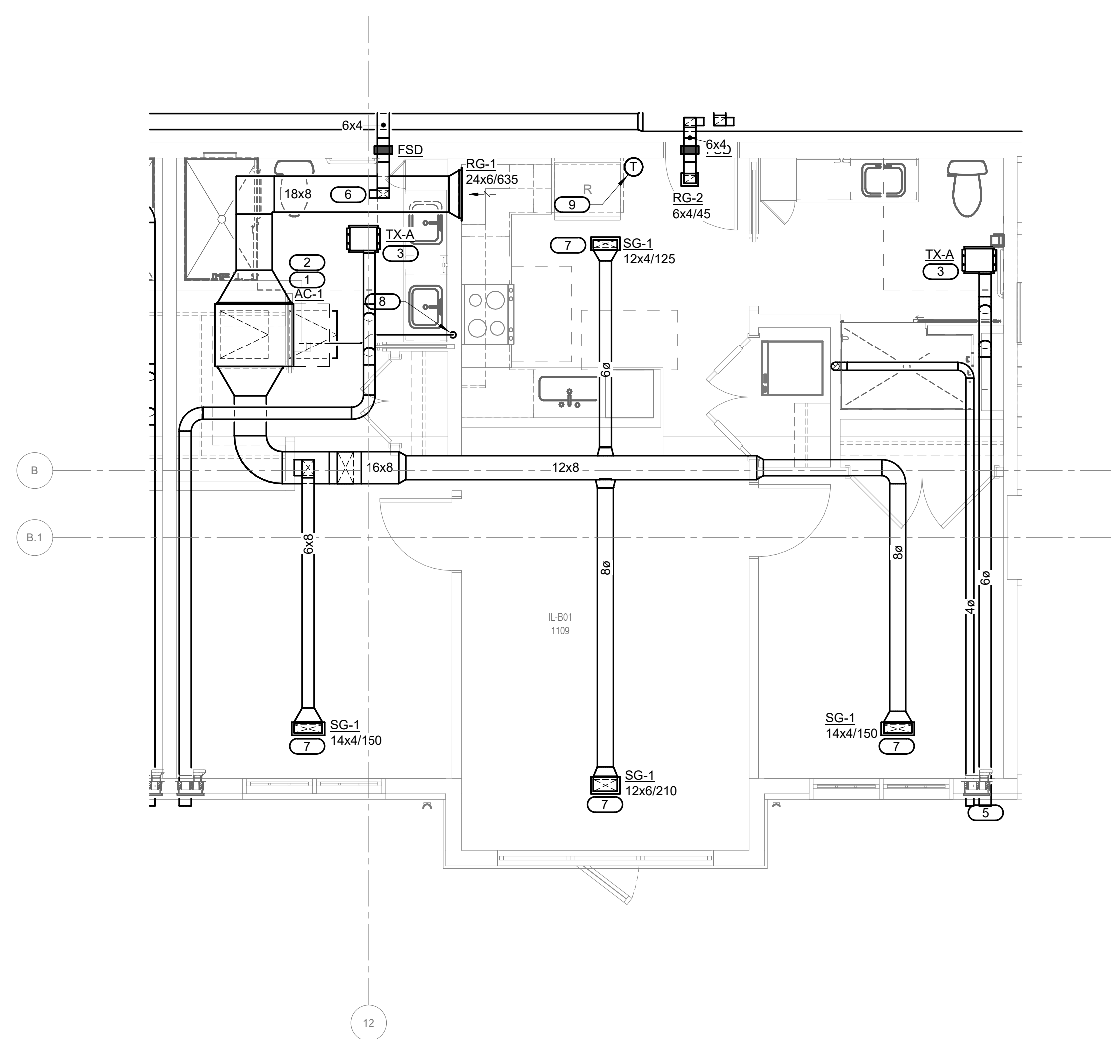
2 MECH. UNIT B01 - 2 BED 2 BATH - PLAN - AC-1 - FIRST FLOOR 1/4" = 1'-0"
