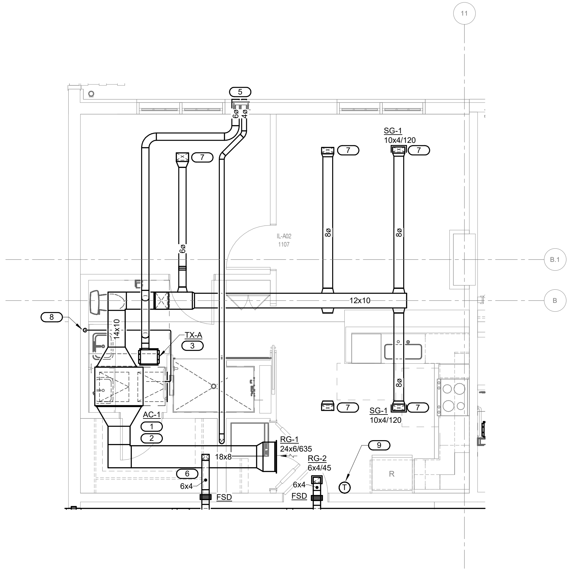
1 MECH. UNIT A02 -1 BED 1 BATH - PLAN - AC- 1 - FIRST FLOOR 1/4" = 1'-0"
