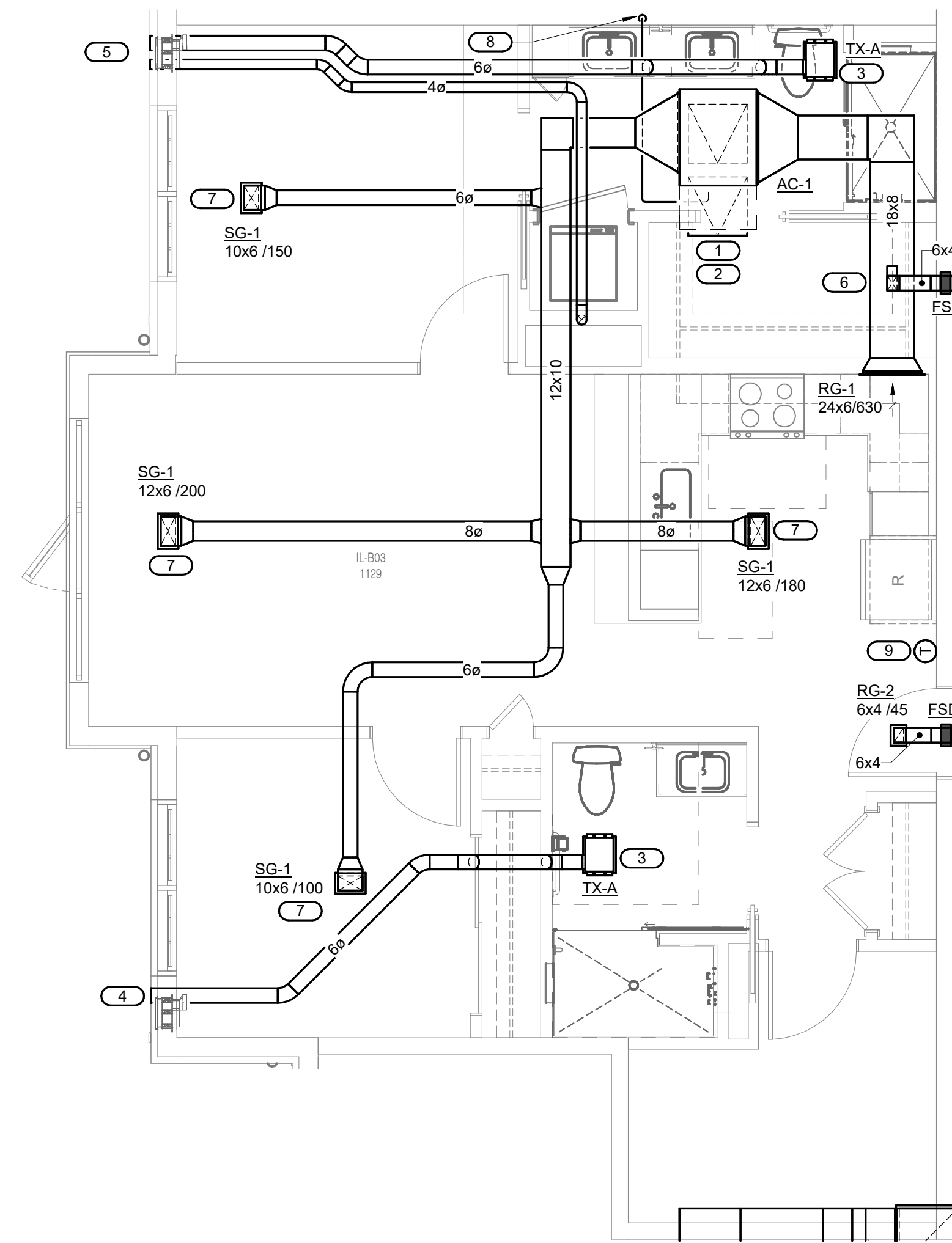
4 MECH. UNIT B03 - 2 BED 2 BATH - PLAN - AC-1 - FIRST FLOOR 1/4" = 1'-0"
