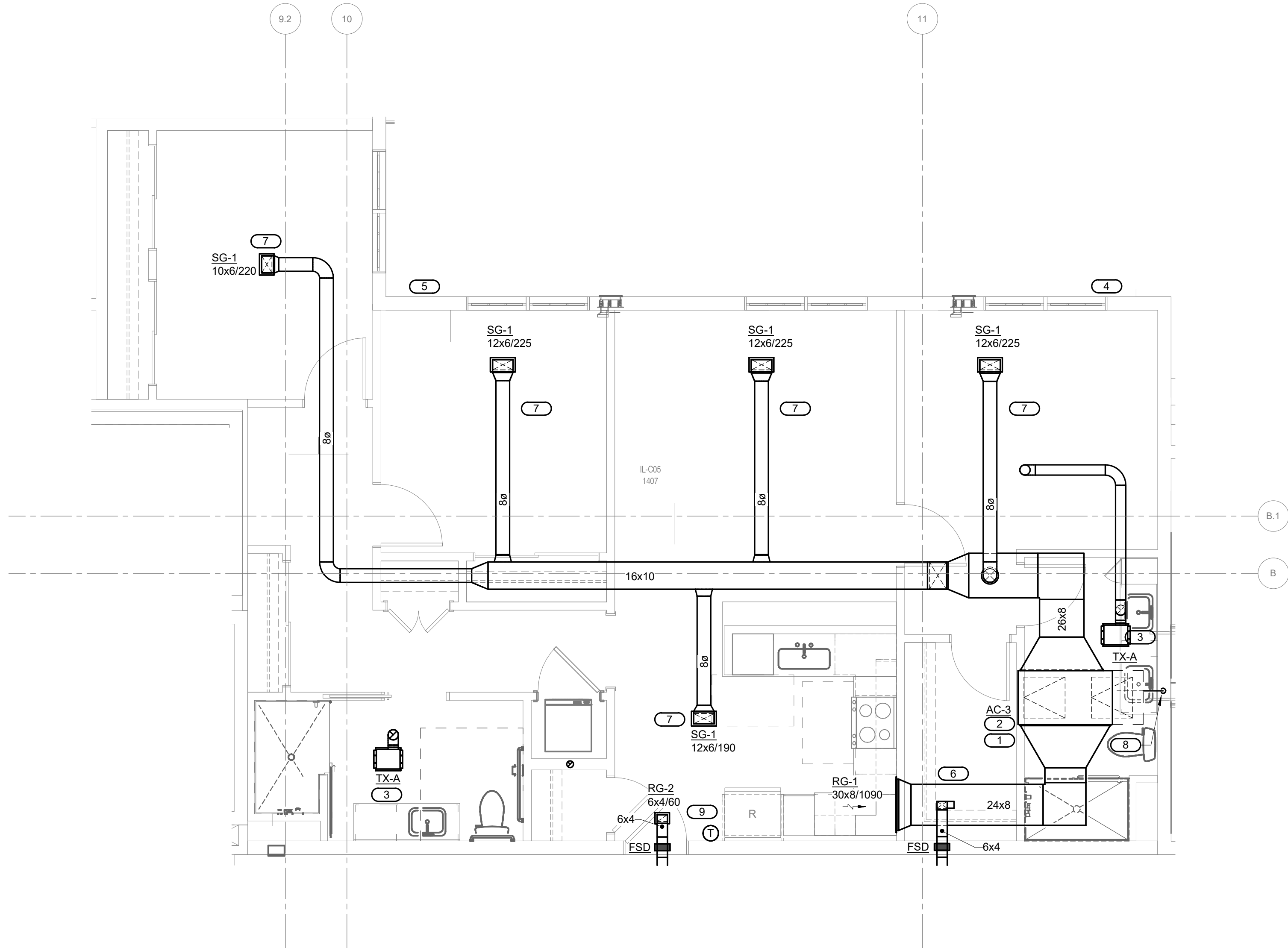
2 MECH. UNIT C05 - 3 BED 2 BATH - PLAN 1/4" = 1'-0"
