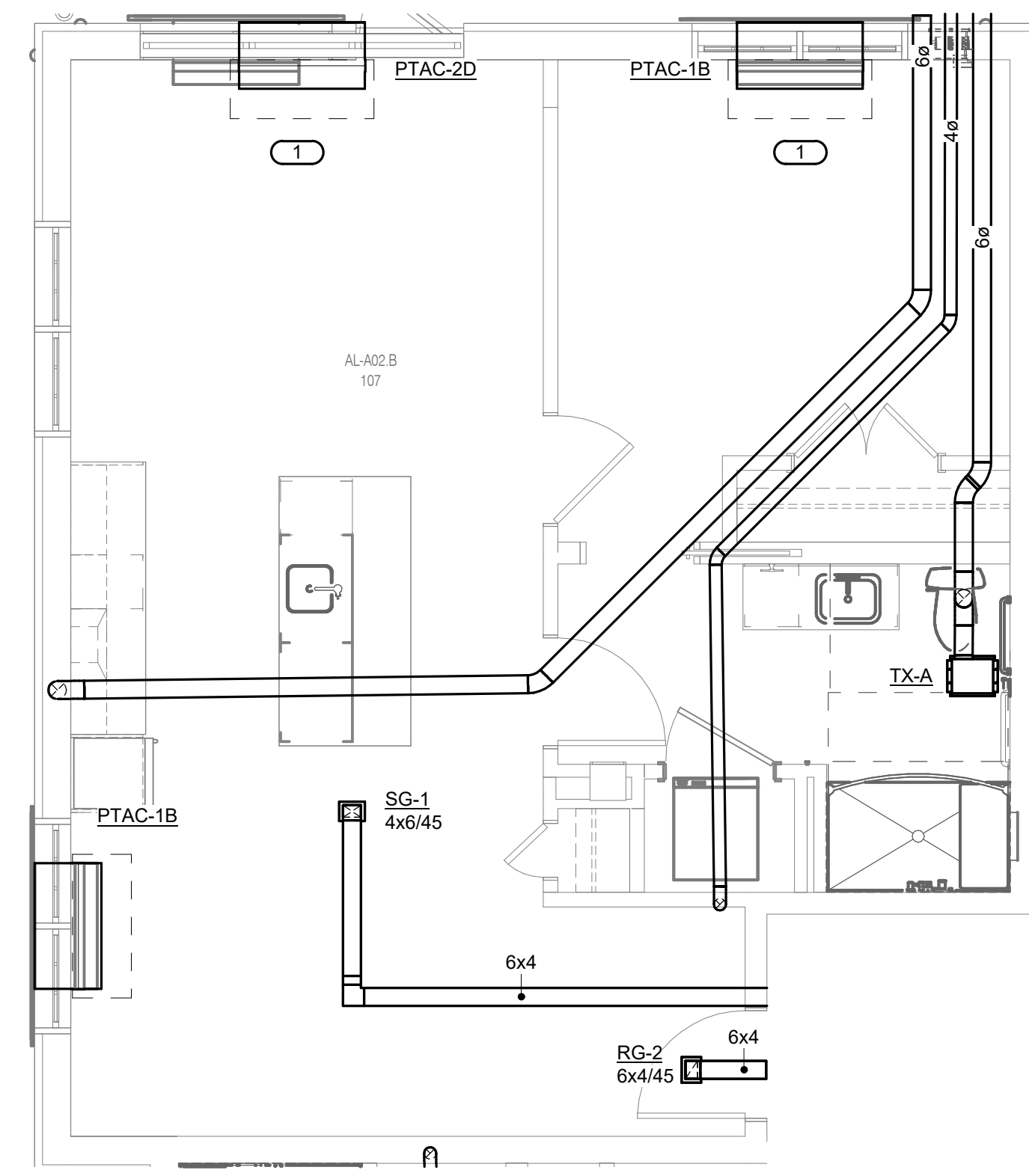
3 MECH. UNIT - (NORTH) CORNER - 1 BED 2 BATH - AL-A02.B 1/4" = 1'-0"
