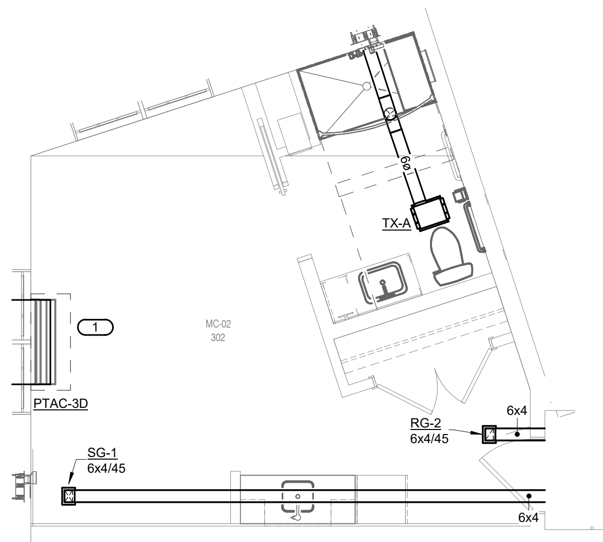
3 MECH. REM - PRIVATE - CORNER UNIT - MC-02 1/4" = 1'-0"
