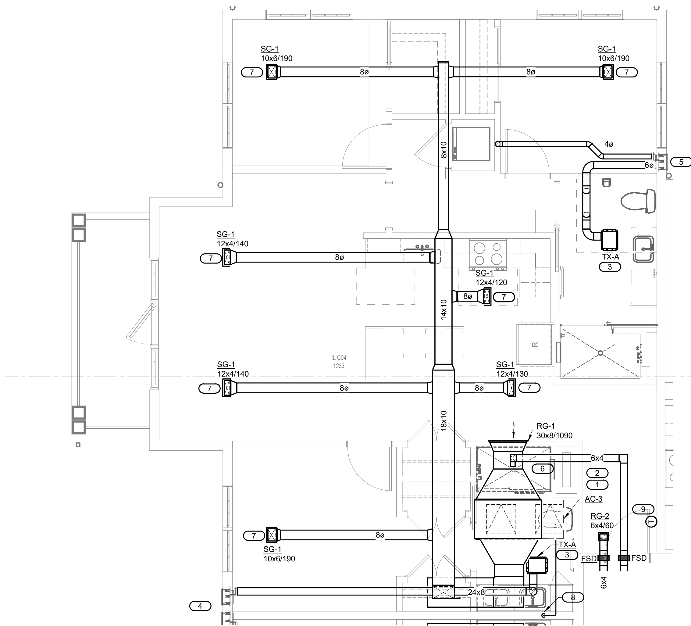
4 MECH. UNIT C04 - 3 BED 2 BATH - PLAN - AC-3 1/4" = 1'-0"
