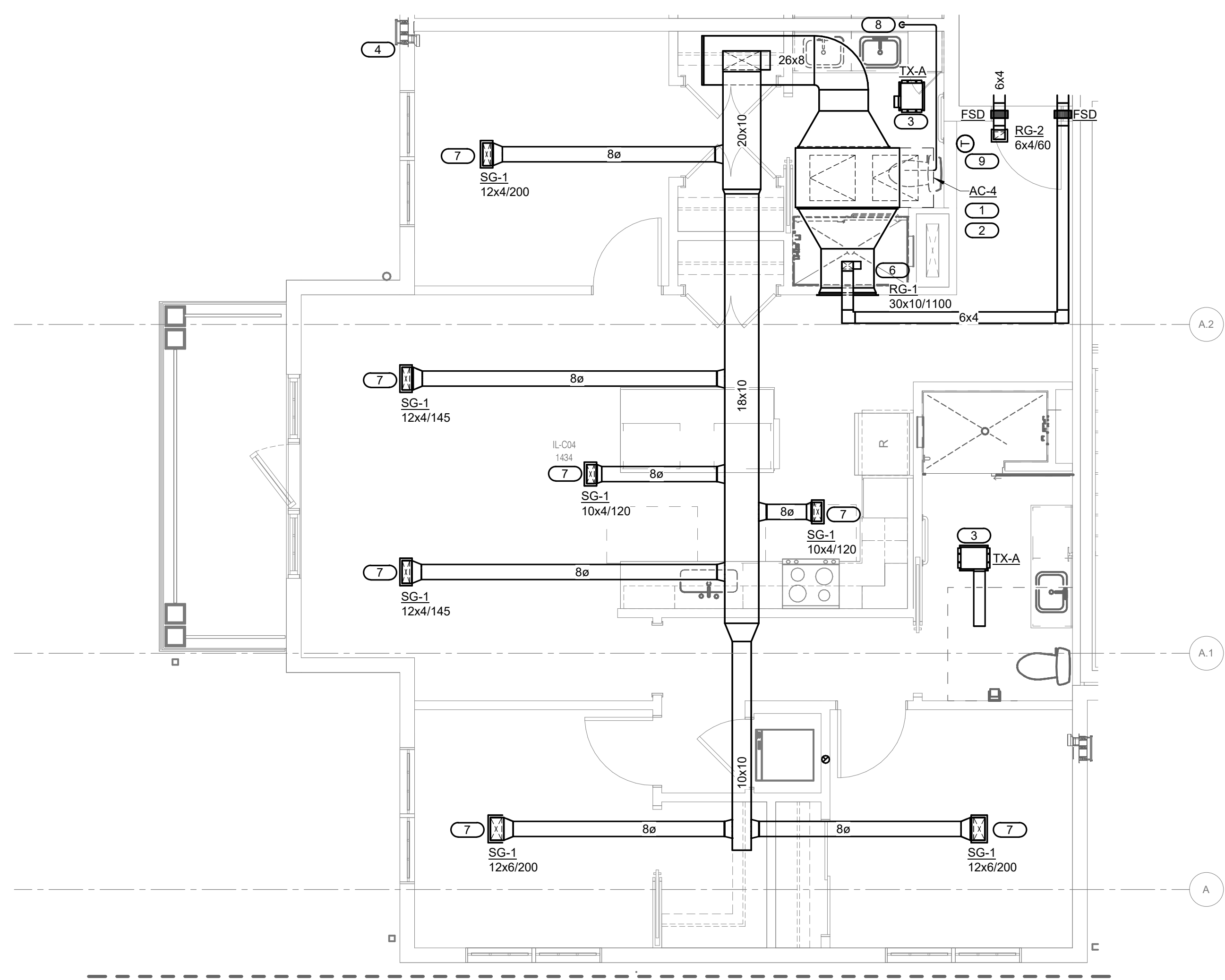
1 MECH. UNIT C04 - 3 BED 2 BATH - PLAN - AC-4 1/4" = 1'-0"
