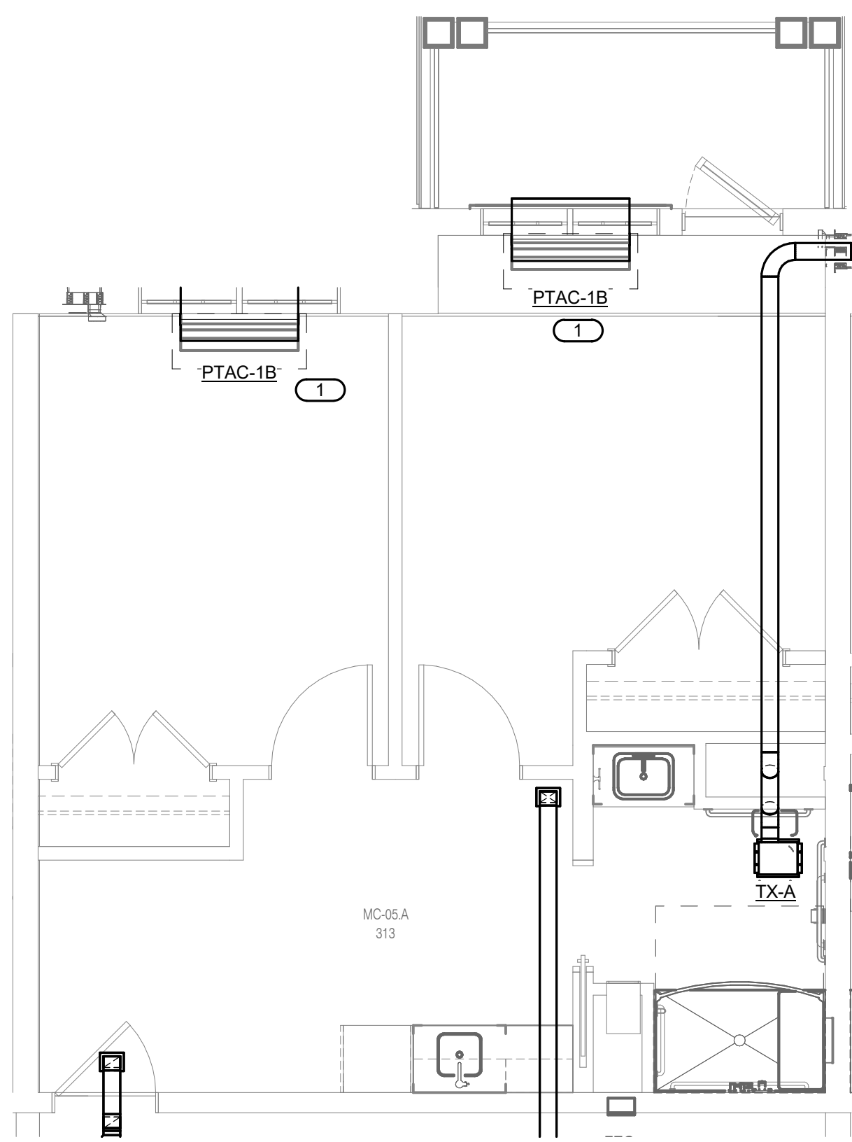
1 MECH. REM SEMI-PRIVATE (TYPICAL) - MC-05 1/4" = 1'-0"
