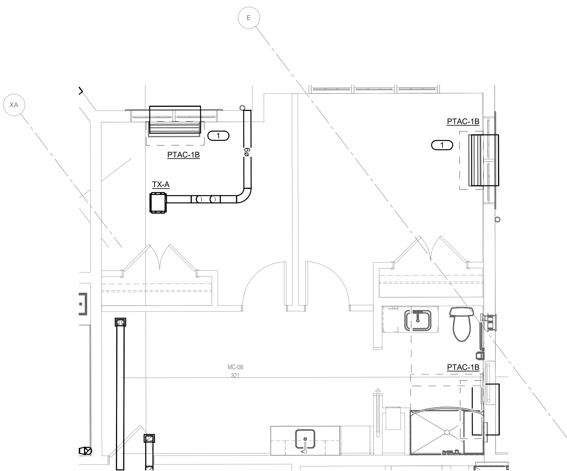
3 MECH. REM SEMI-PRIVATE - MC-08 1/4" = 1'-0"
