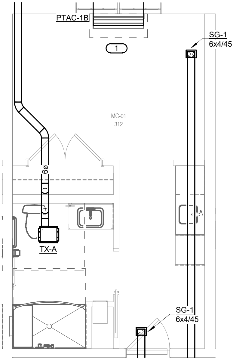
2 MECH. REM - PRIVATE (TYPICAL) - MC-01 1/4" = 1'-0"
