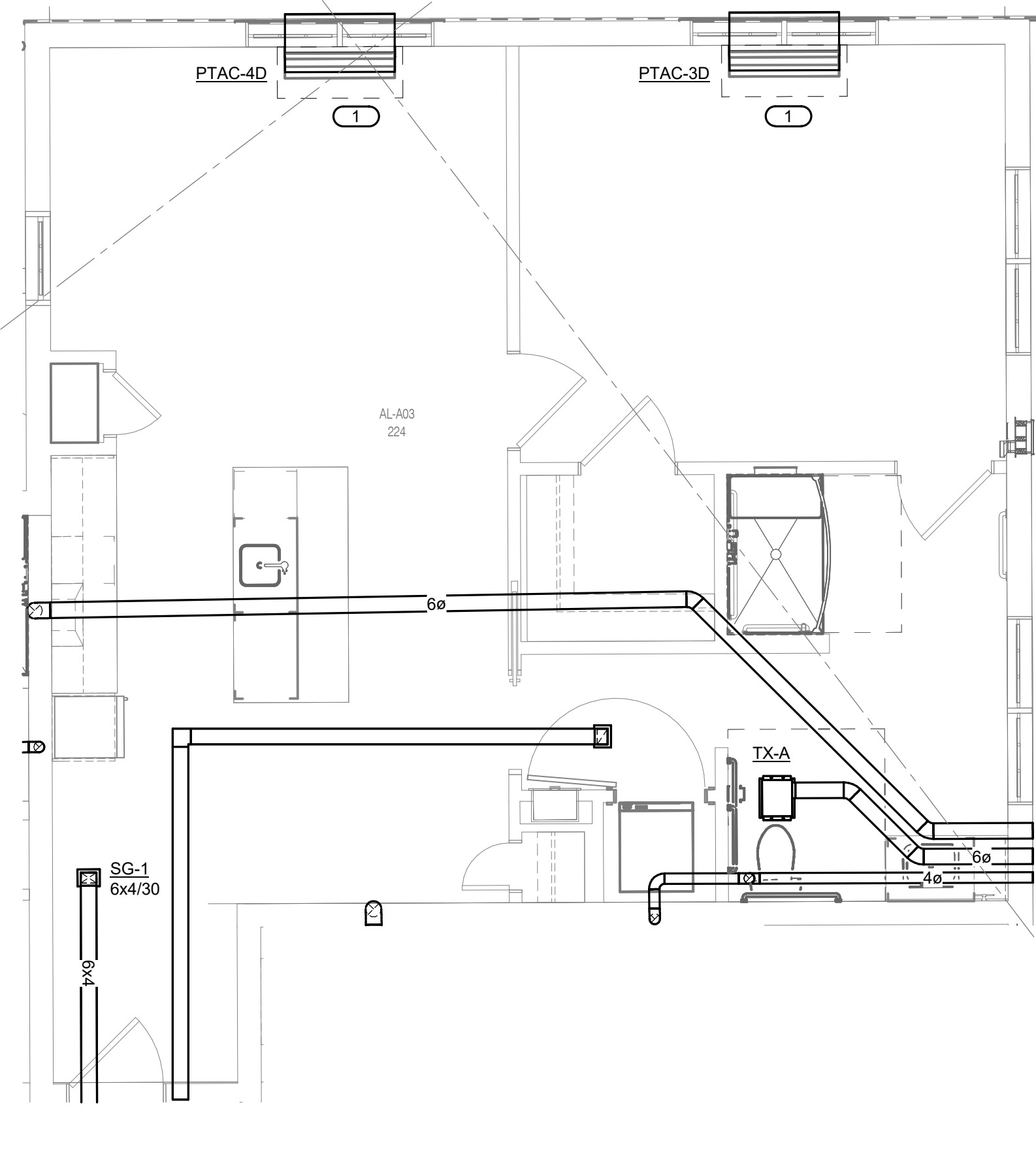
4 MECH. UNIT - 1 BED 1 BATH - AL-A03 1/4" = 1'-0"
