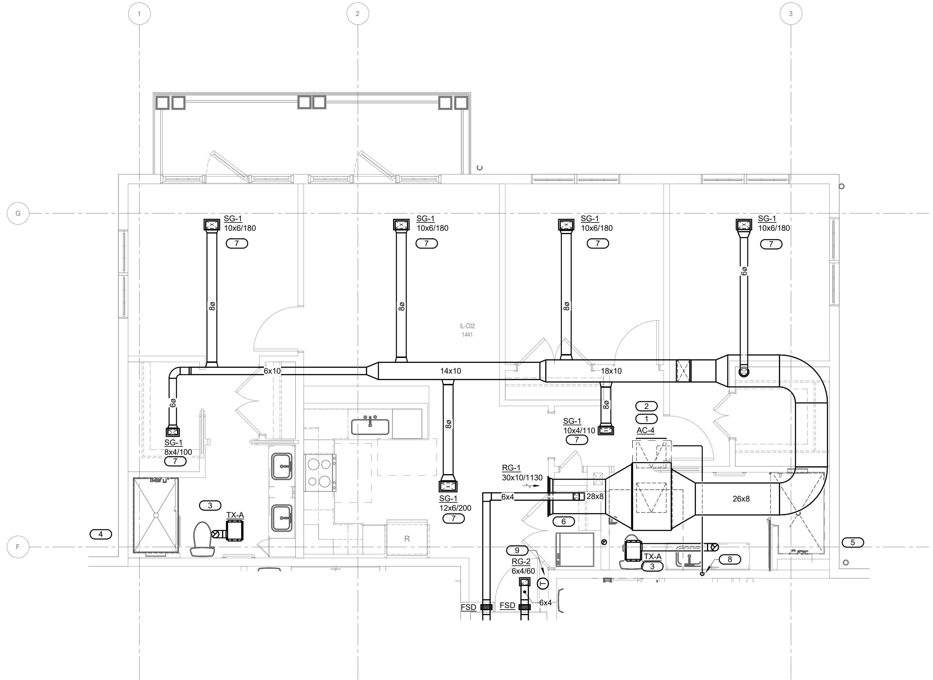
1 MECH. UNIT C02 - 3 BED 2 BATH - PLAN - AC-4 1/4" = 1'-0"
